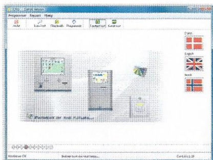
iCHIP program
