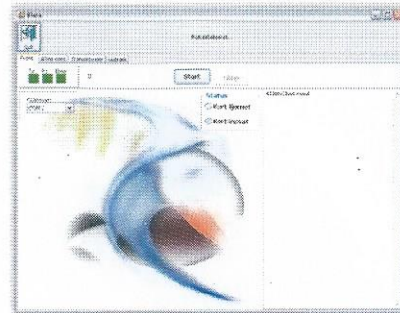
iDATA program
